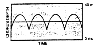
CHORUS WAVEFORM: LOGARITHMIC
