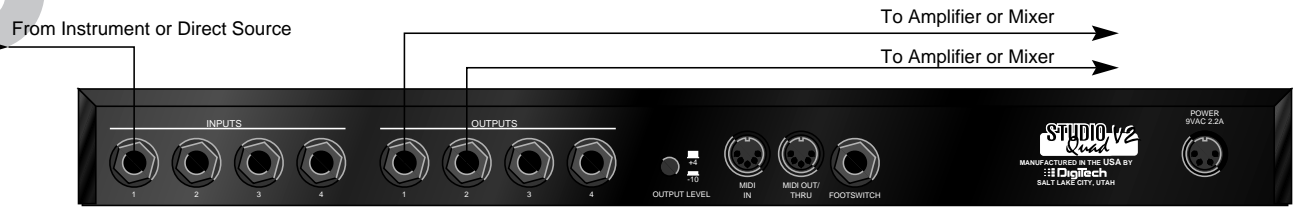
Figure I-3 In-Line Connection
