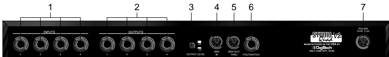
Figure I-2 Rear Panel
