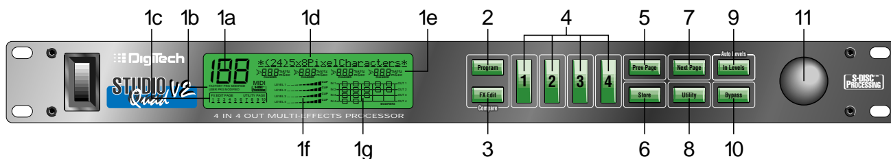
Figure I-1 Front Panel
